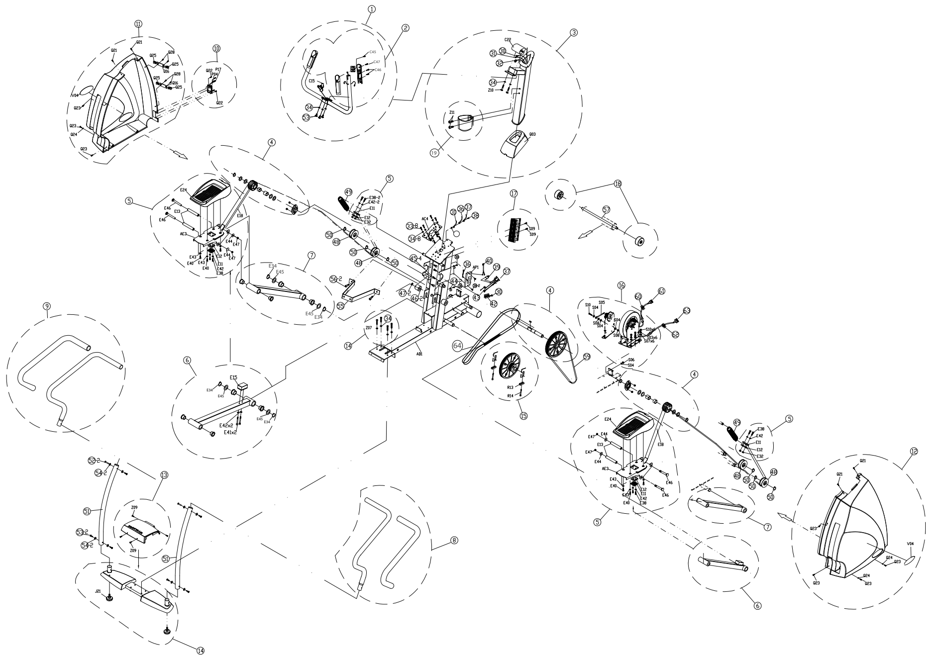
Service Drawing of Matrix S5x-F
